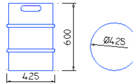
KEG - FASS 50 L EURO-NORM
